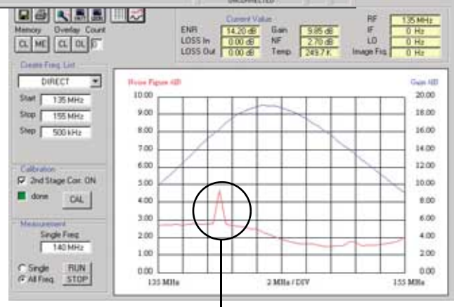
Fast and simple analysis of anomalies. The cause – spurious or RFI – can easily be traced with the basic analyzer function without additional measuring equipment.
