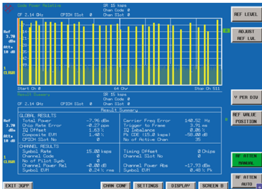
WCDMA code domain power measurement with R&S FSQ and R&S FS-K72
